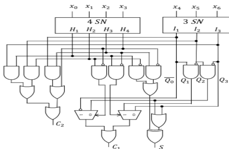
Fig:3 Overall (7,3) counter circuit
