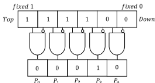
Fig. 7 One-hot code generation circuit.
