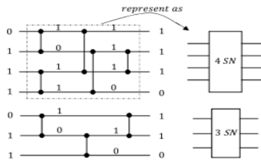
Fig.4 Three- and four-way sorting networks.
