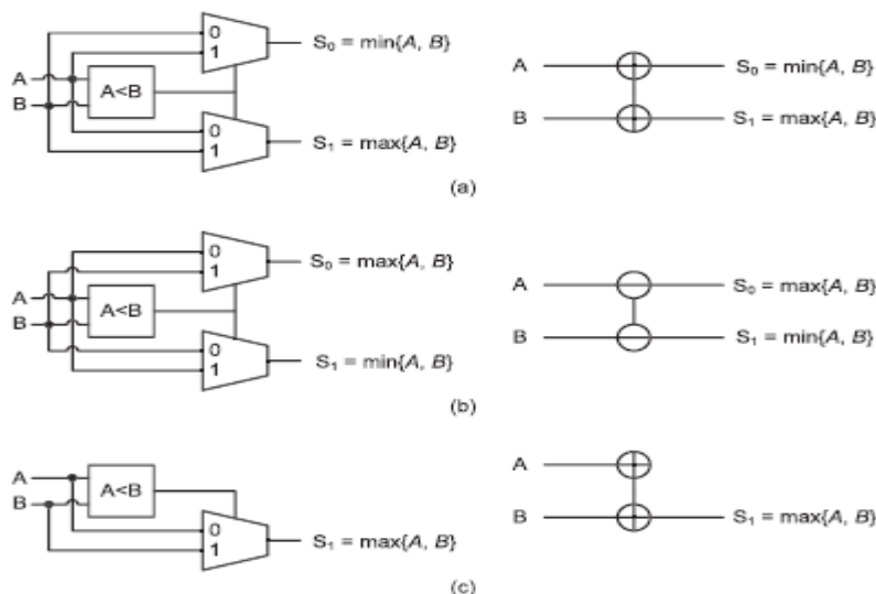
Fig:2parallel sorting units
