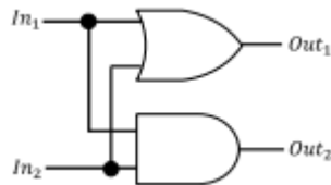
Fig.5 Two-input binary sorter
